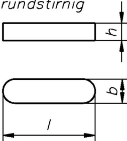
Feather key form A height 6mm 1673/000/99 6x20
